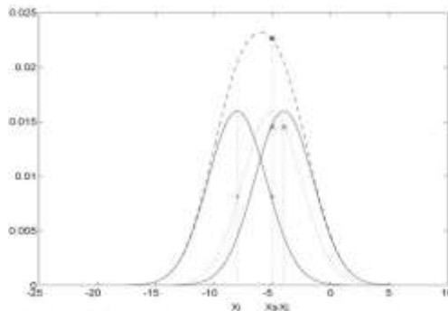
Fig. 1. One kernel at x_5 ( dotted kernel ) or two kernels at x_i and x_j ( left and right ) lead to the same summed estimate at x_5 . This shows a figure consisting of different types of lines. Elements of the figure described in the caption should be set in italics, in parentheses, as shown in this sample caption.
